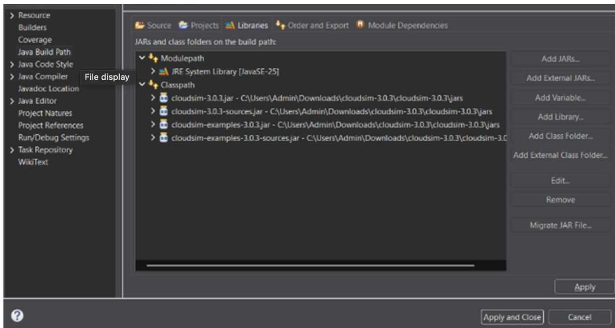
Fig 1.3: CloudSim Project
